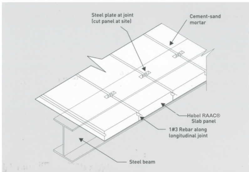
Fig. 19: Cantilever Panel Anchorage
