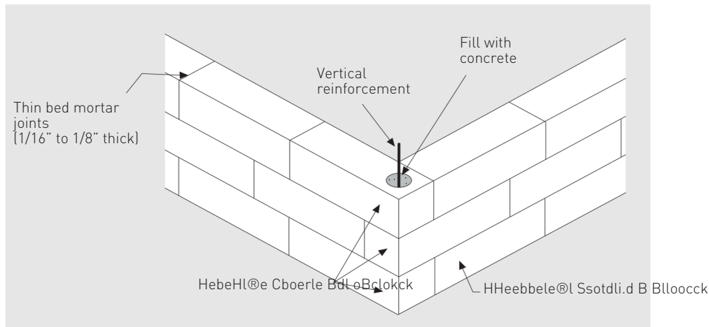
Fig. 11: Pilaster located at corner
